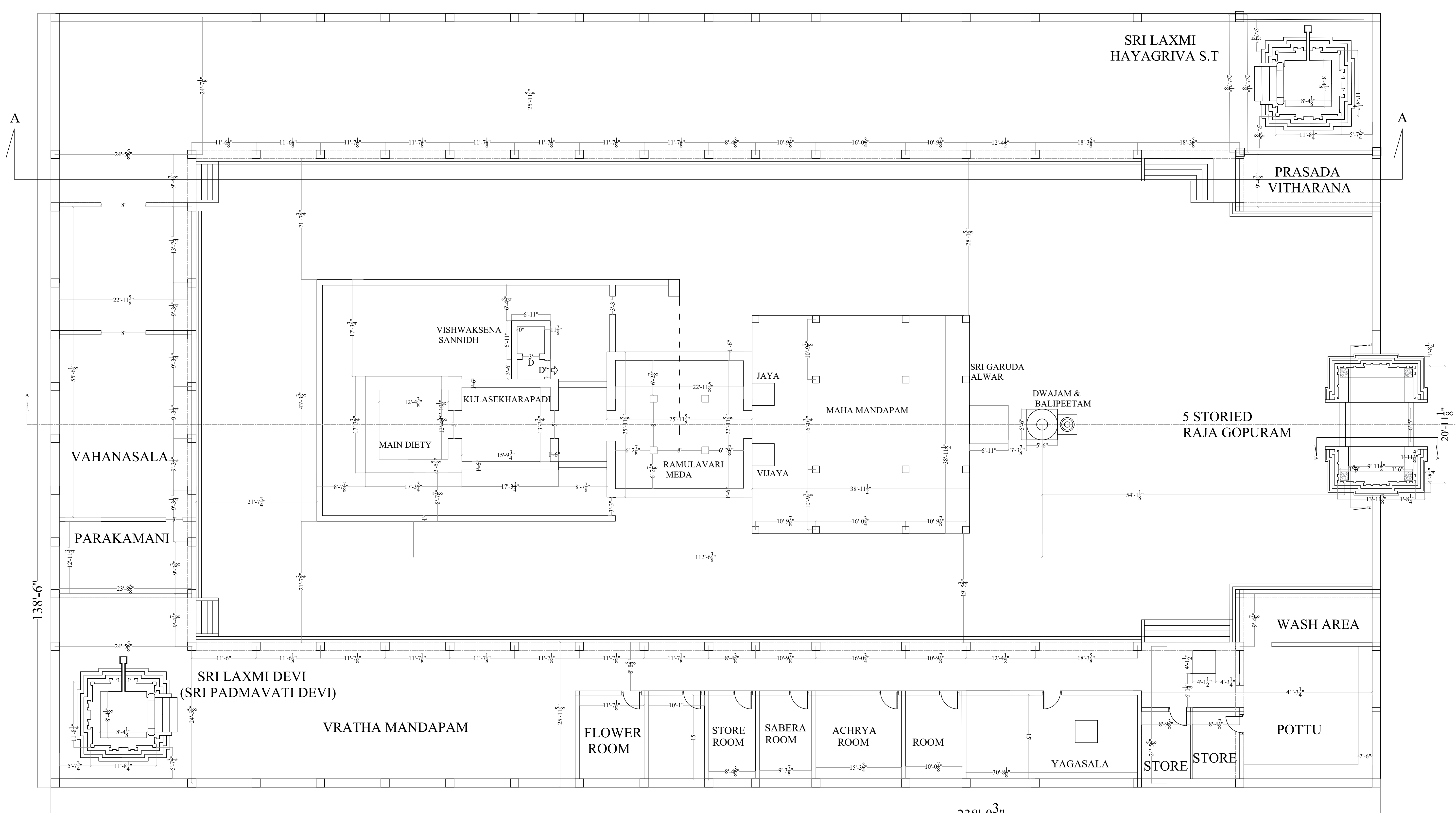
GROUND PLAN
